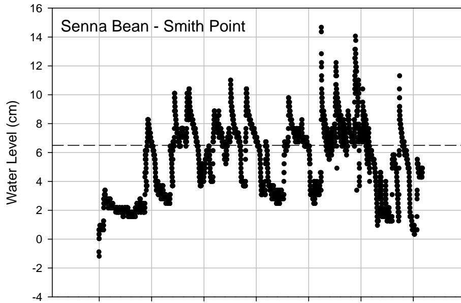
Figure V.5 Hydrograph for Senna Bean Pond (SE) and approximate spill point elevation.
