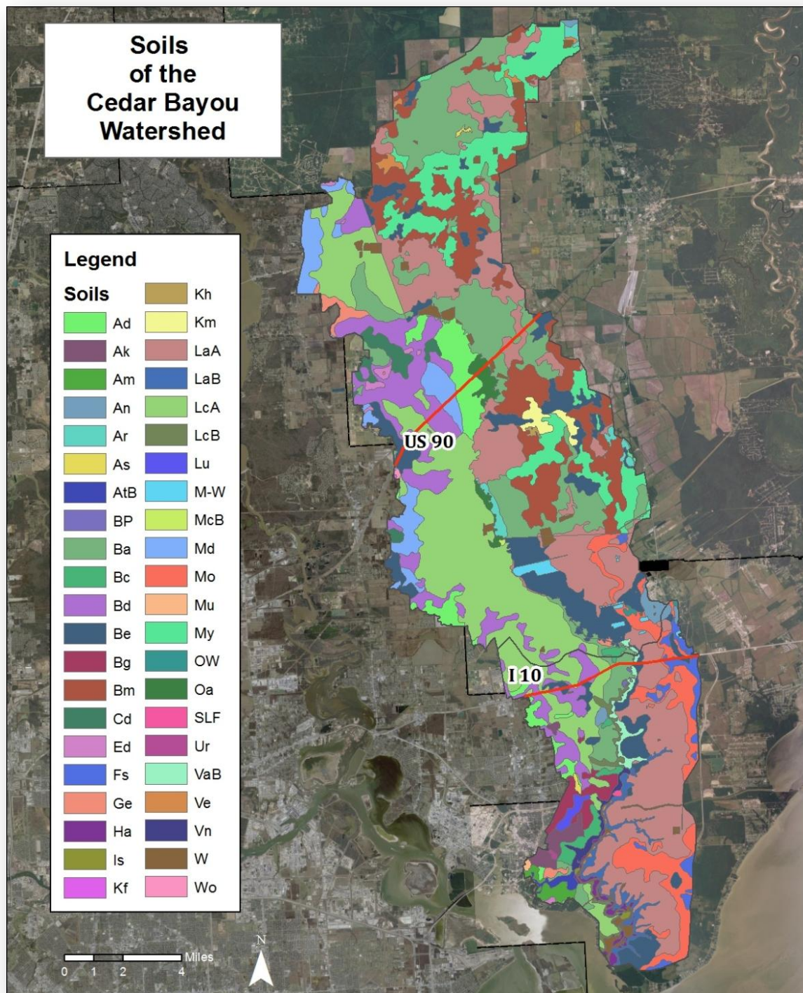
Figure 18 – Soils of the Cedar Bayou Watershed 6
