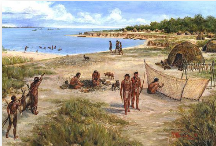
Figure 21 – Indigenous peoples (image courtesy of texasbeyondhistory.net )
