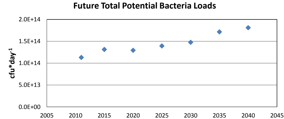
Figure 94 – Total potential bacteria loads over time
