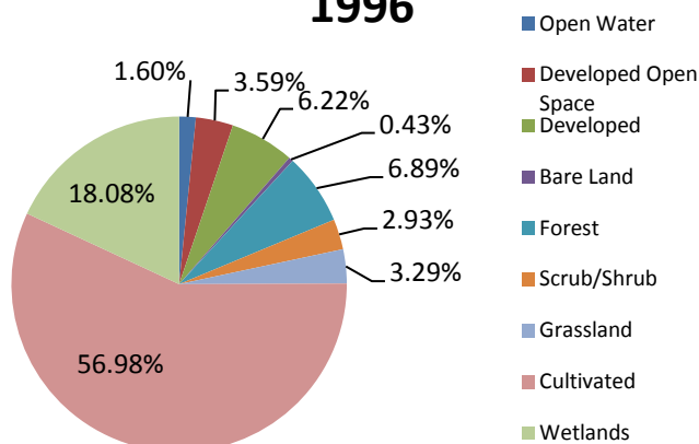
Figure 35 – Cedar Bayou land cover, 1996
