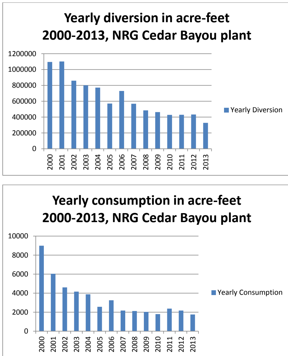
Figure 28 – NRG yearly diversion and consumption, 2000-2013
