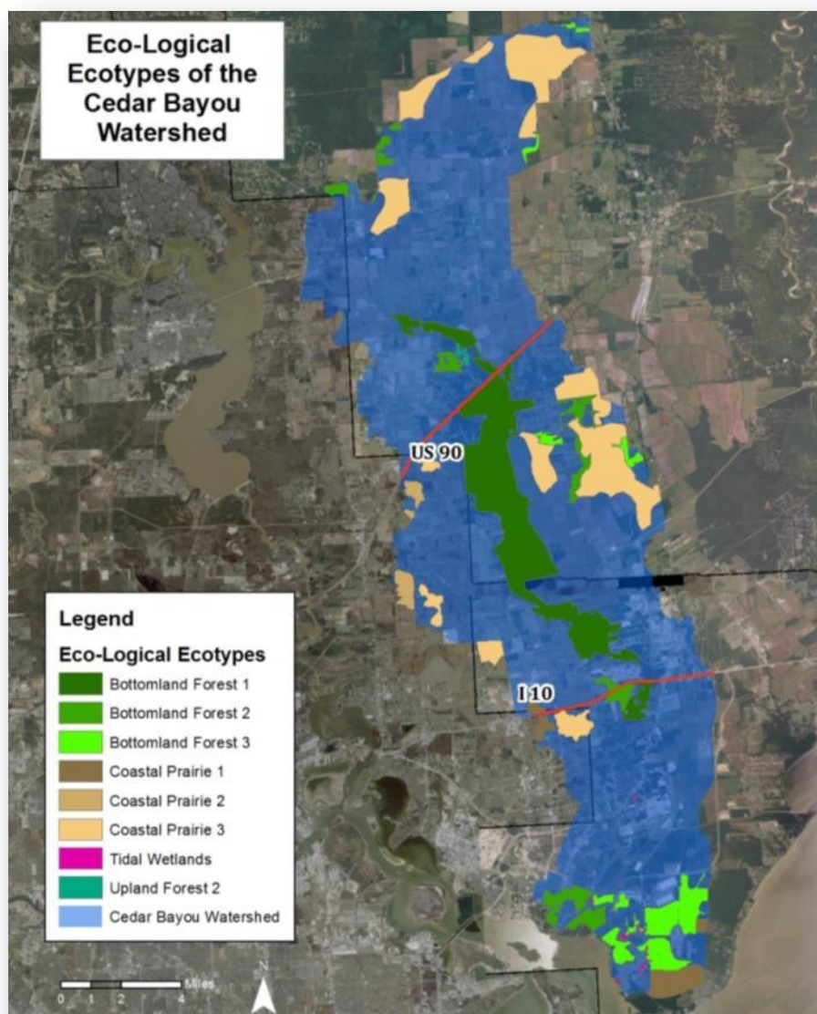
Figure 20 – Eco-Logical ecotypes of the Cedar Bayou Watershed.
