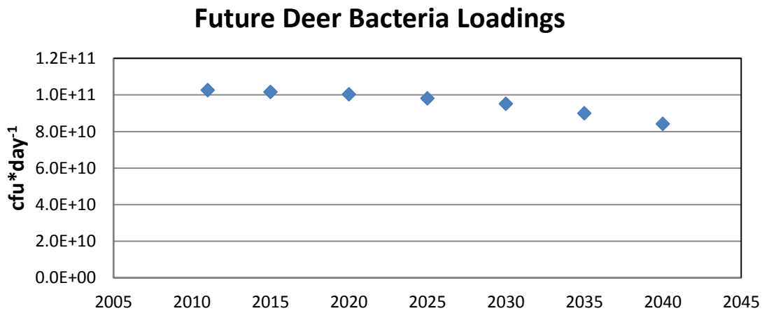
Figure 79 – Future bacteria loads from deer
