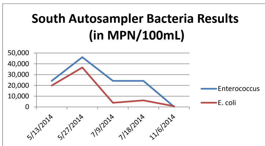
Figure 99 – South autosampler bacteria results
