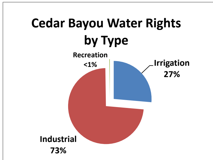
Figure 27 – Cedar Bayou surface water rights, by type
