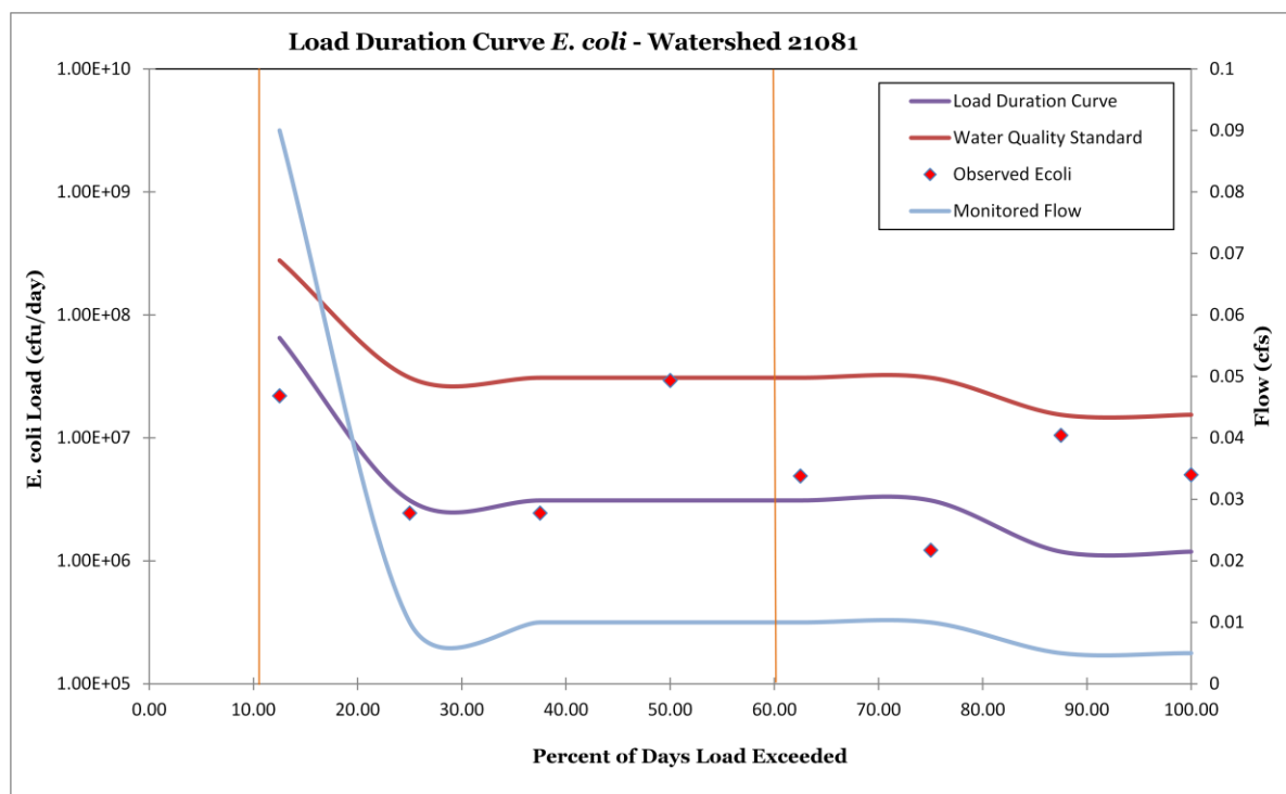
Figure 39 – LDC for station 21081
