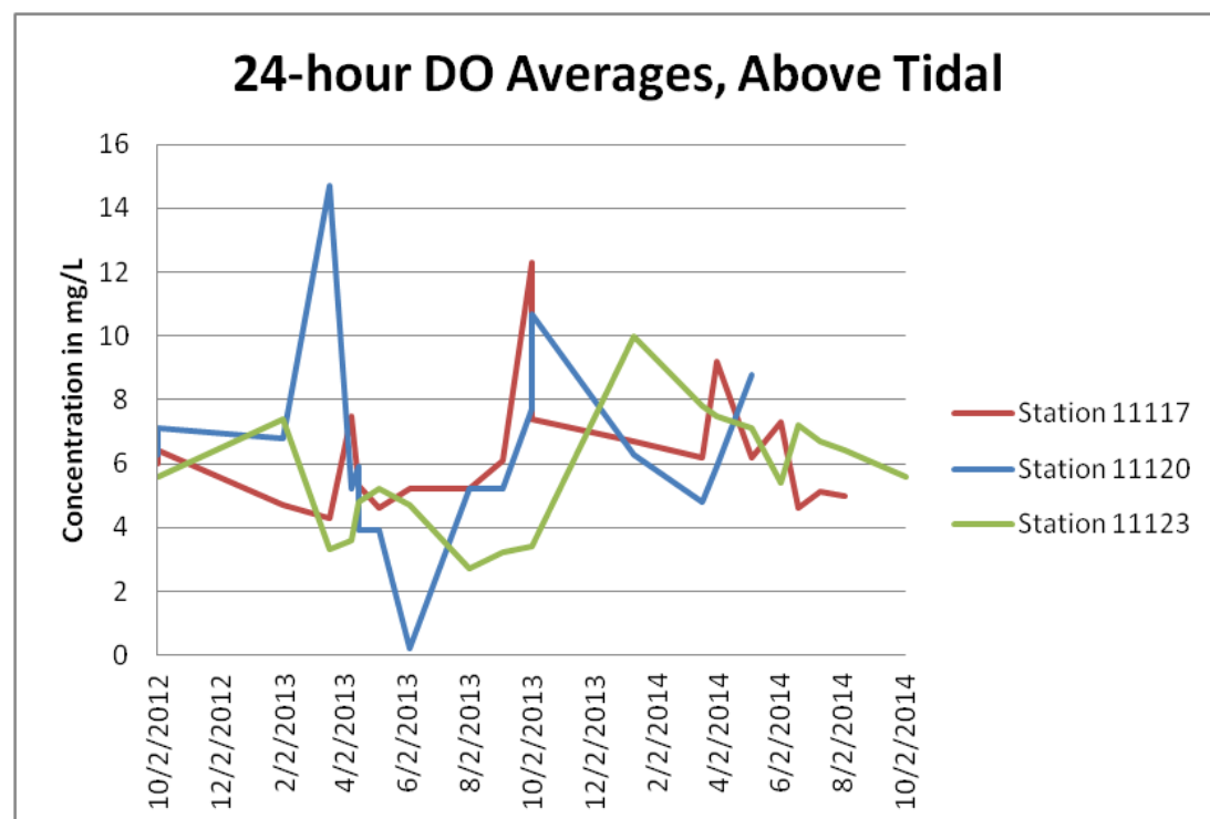
Figure 97 – 24-hour DO average values
