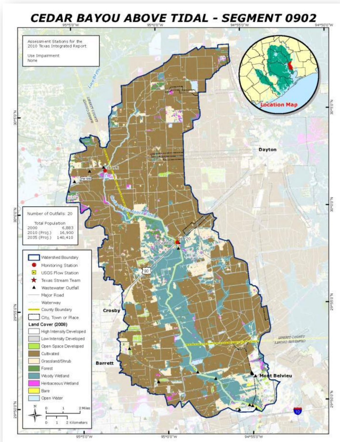
Figure 10 – Land use map of Cedar Bayou Above Tidal (Segment 0902)
