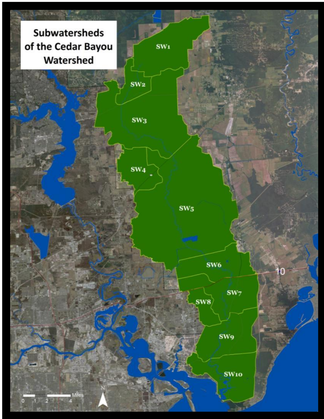
Figure 15 – Subwatersheds of the Cedar Bayou Watershed 3
