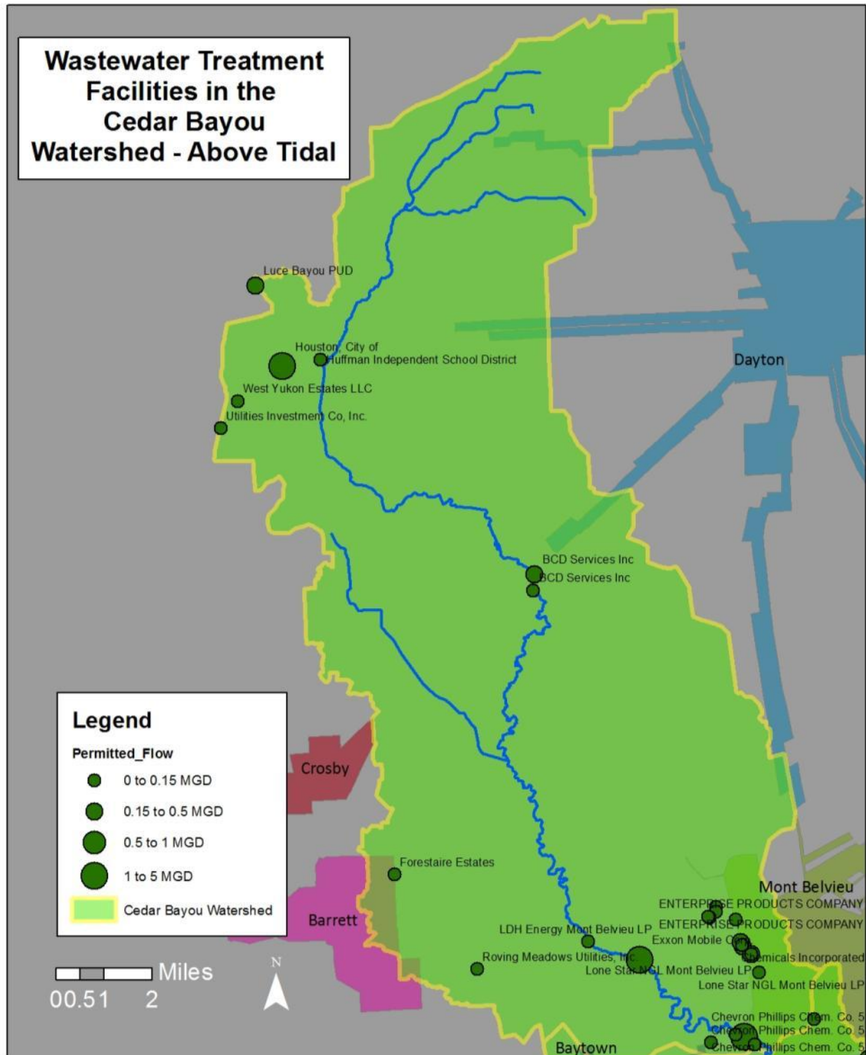
Figure 70 –WWTFs in the Above Tidal segment
