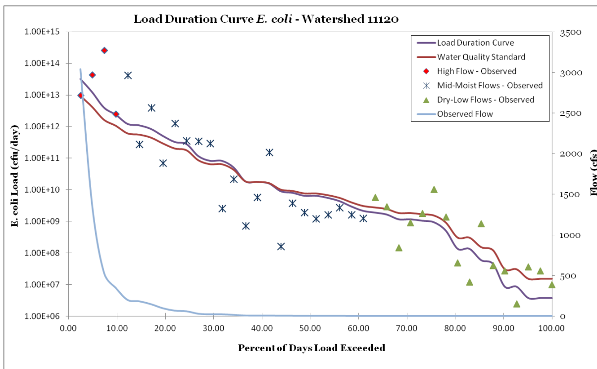
Figure 43 – LDC for station 11120
