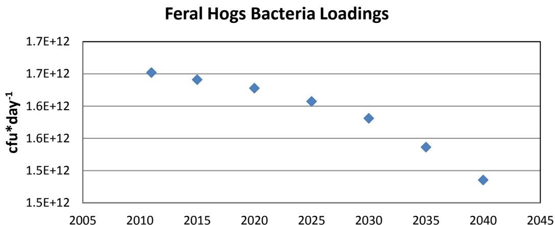
Figure 84 – Future bacteria loadings from feral hogs
