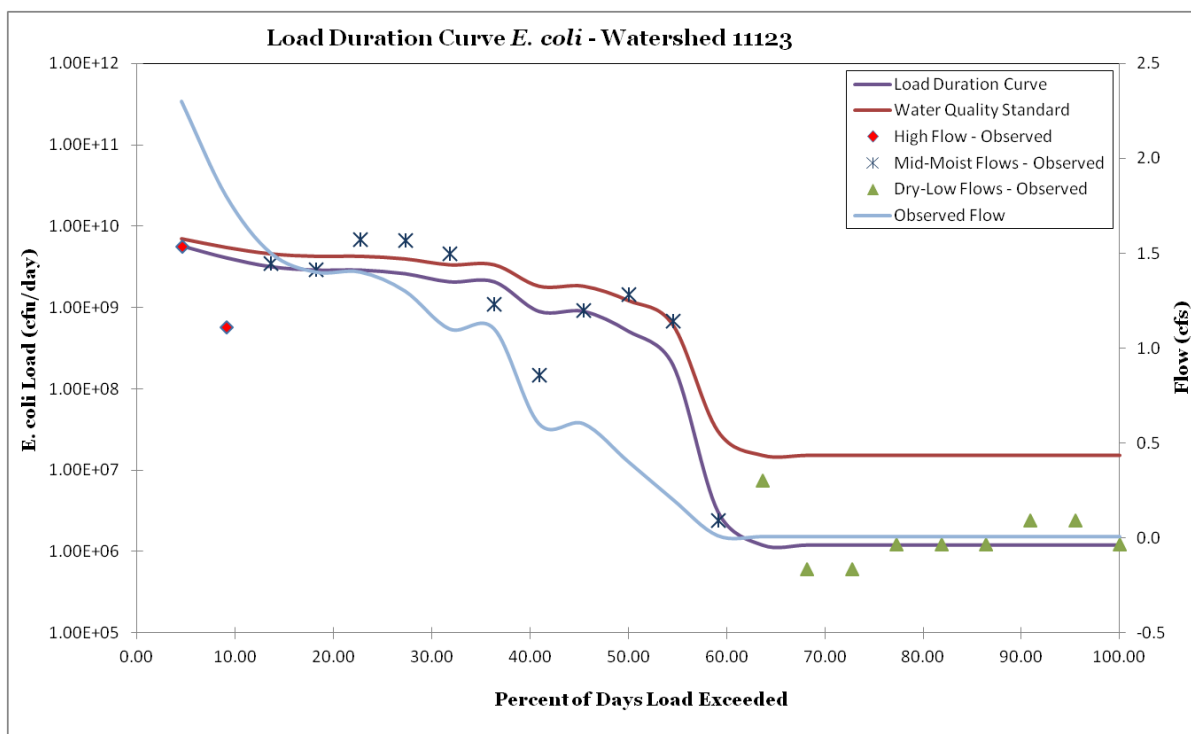
Figure 41 – LDC for station 11123
