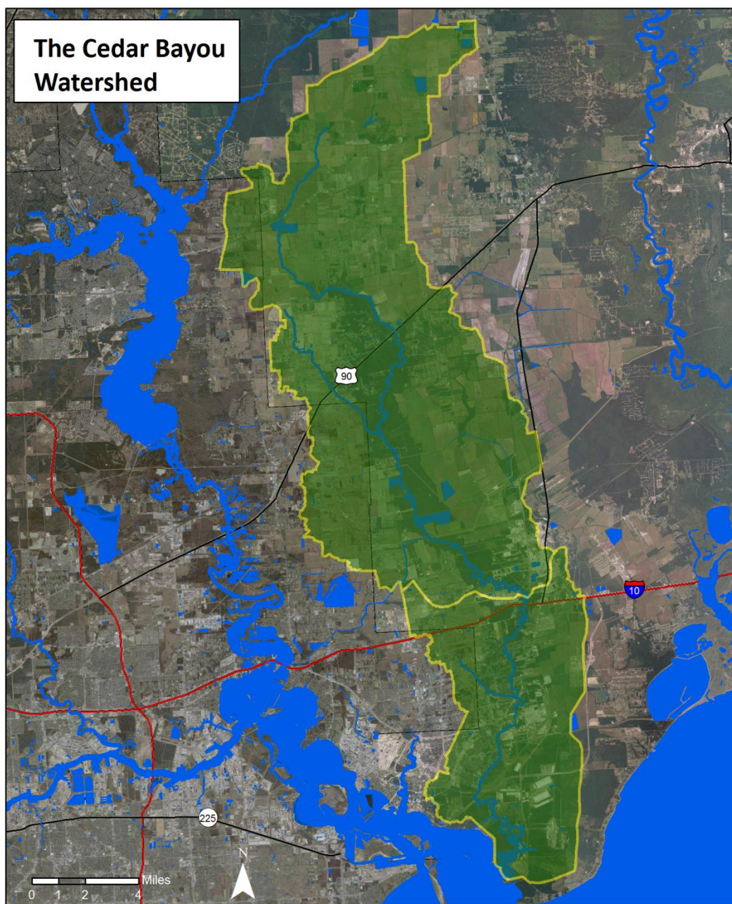
Figure 14 – Cedar Bayou watershed project area
