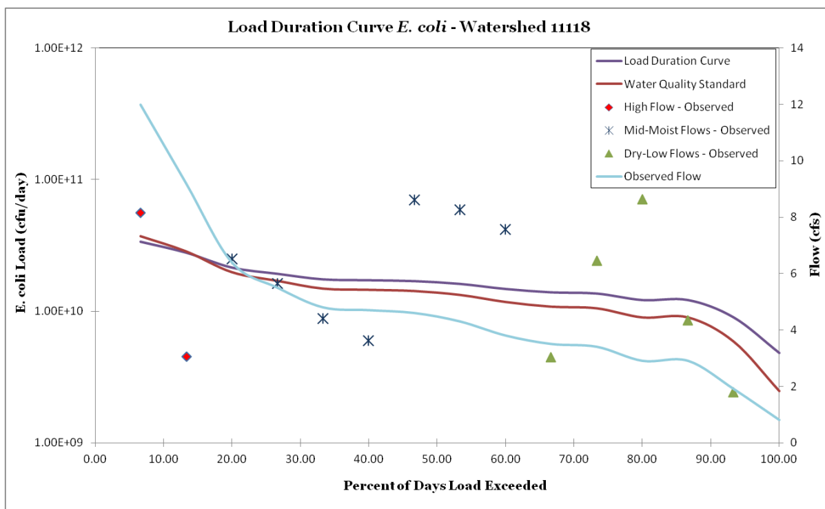
Figure 45 – LDC for station 11118
