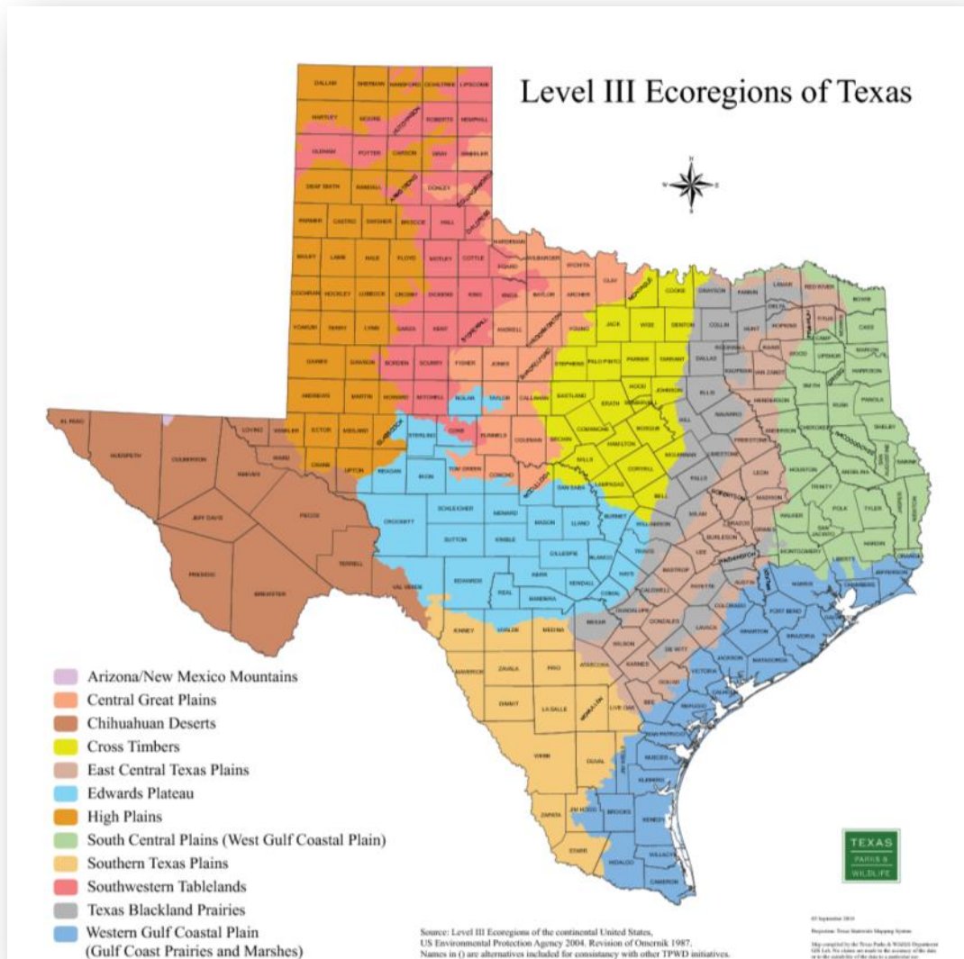
Figure 19 – Level III Ecoregions of Texas
