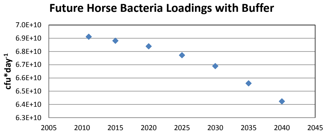
Figure 59 – Future bacteria loads from horses (Buffered)
