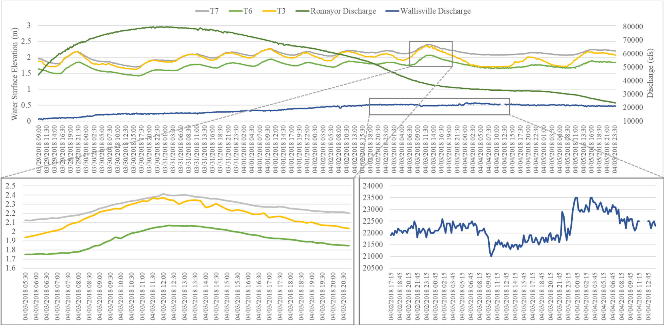
Figure 26. Zoomed-in view of the freshwater inflow event that occurred before the first Atlantic Rangia field sampling. Water surface elevation (m) measured at the three study sites (T3, T6, and T7) and discharge (cfs) from the USGS sites Trinity River at Wallisville (08067252) and Trinity River at Romayor (08066500). Sub-graphs show peaks at the water surface elevation study sites and the Wallisville gage.
