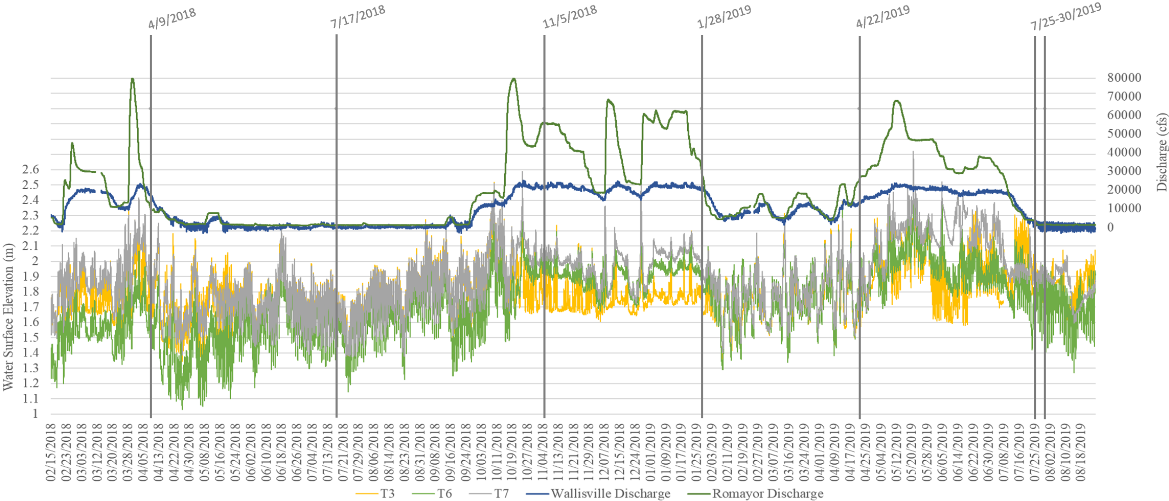
Figure 25. Water surface elevation (m) measured at three study sites (T3, T6, and T7) and discharge (cfs) from the USGS sites Trinity River at Wallisville (08067252) and Trinity River at Romayor (08066500). Vertical demarcations represent Atlantic Rangia sampling events.
